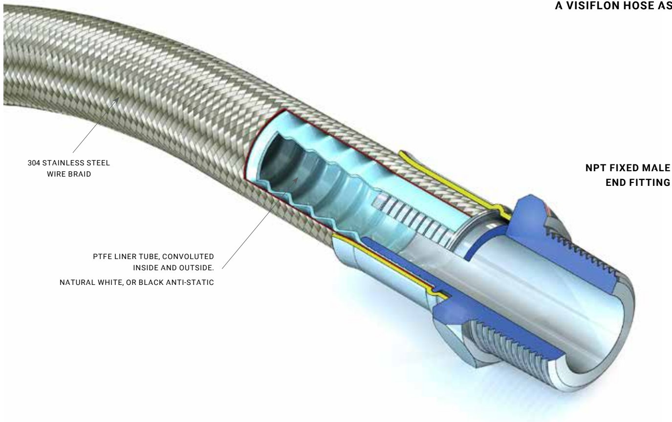
A VISIFLON HOSE ASSEMBLY
