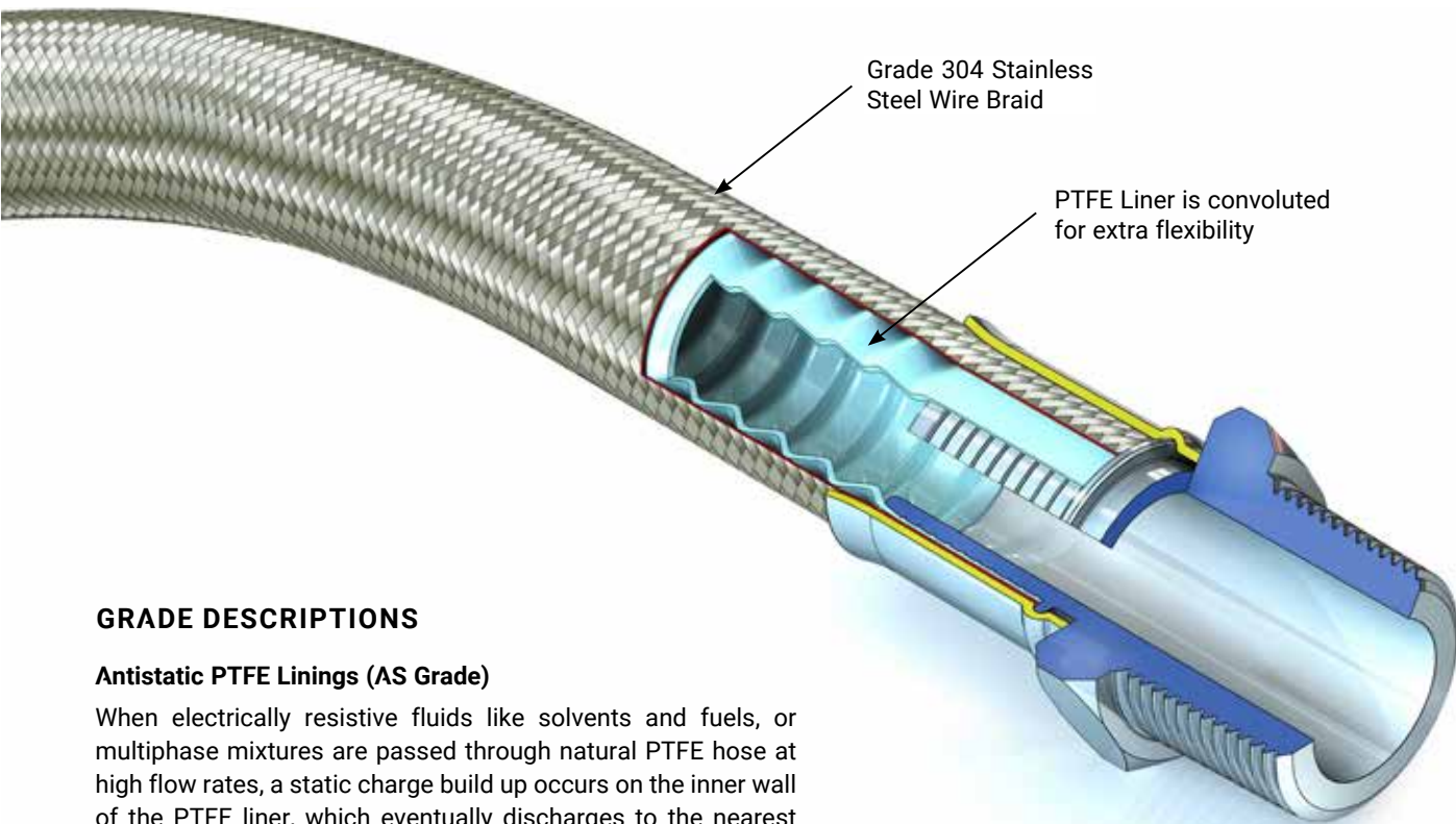
VISIFLON HOSE ASSEMBLY WITH A FIXED MALE END FITTING CRIMPED ON TO THE HOSE
