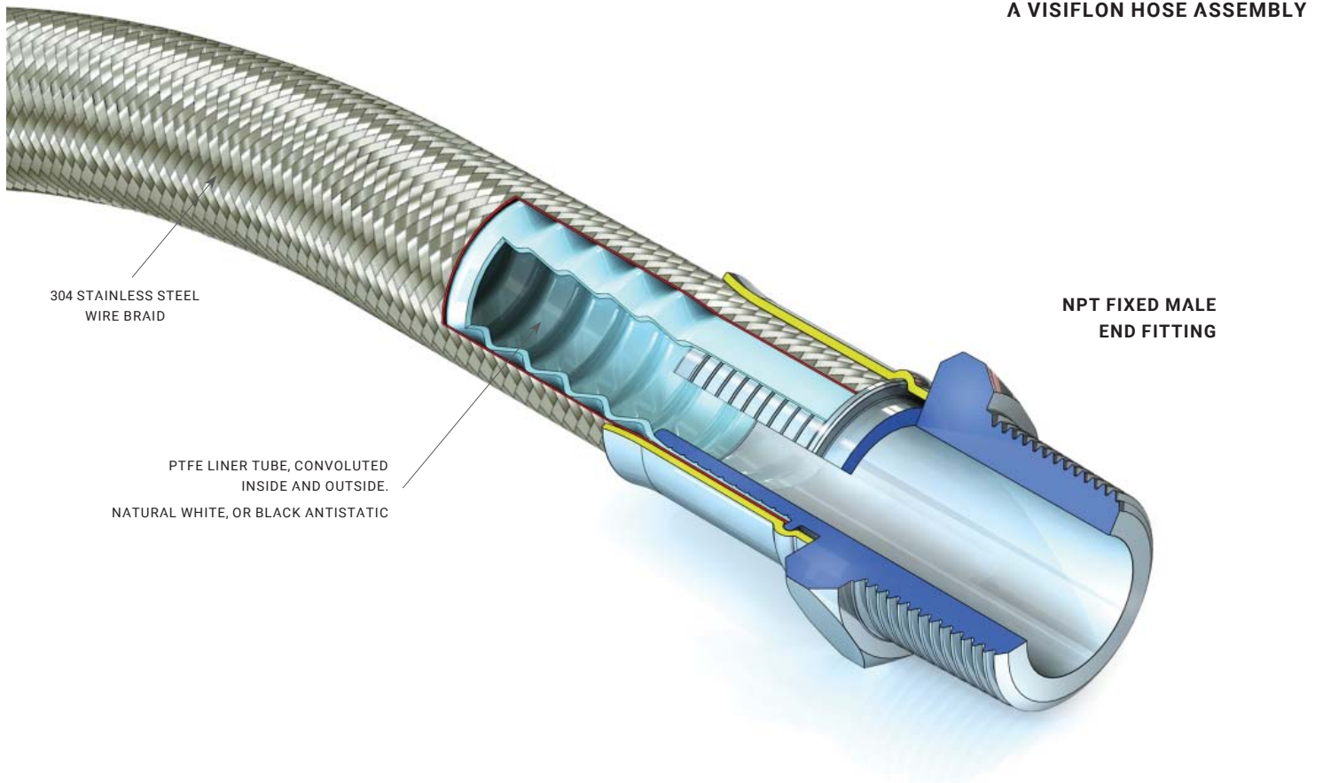
A VISIFLON HOSE ASSEMBLY
