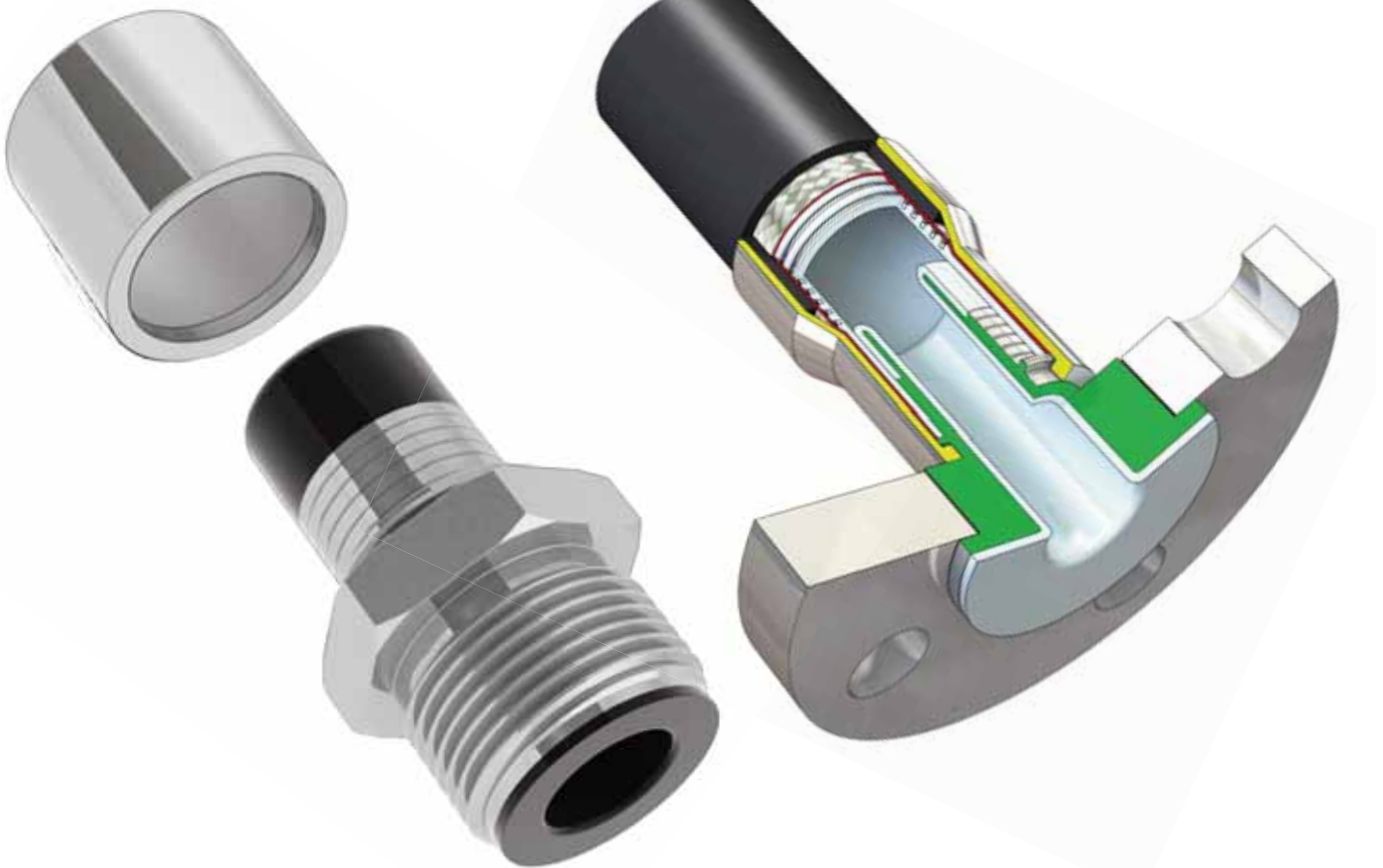
Loose BSPP Fixed Male Encap Fitting and a standard, non-lined Ferrule
